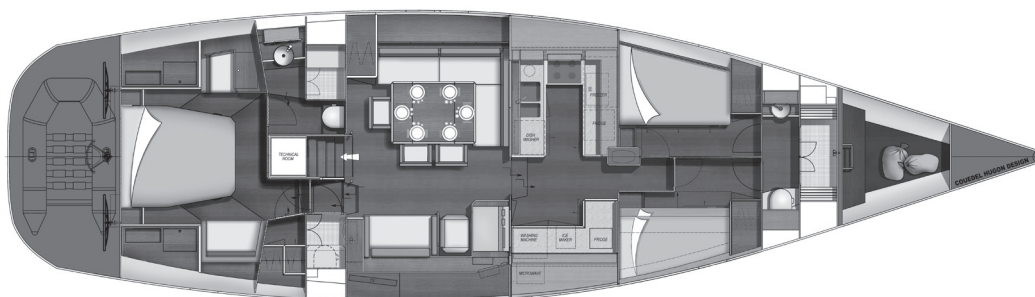
4 - AFT OWNER'S CABIN LAYOUT
