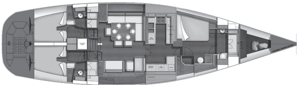
1 - FORWARD OWNER'S CABIN WITH LATERAL BED LAYOUT
