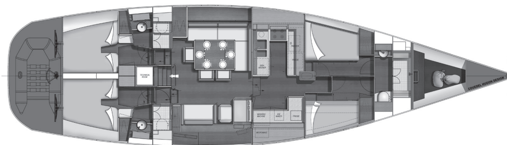
3 - 4 CABIN LAYOUT
